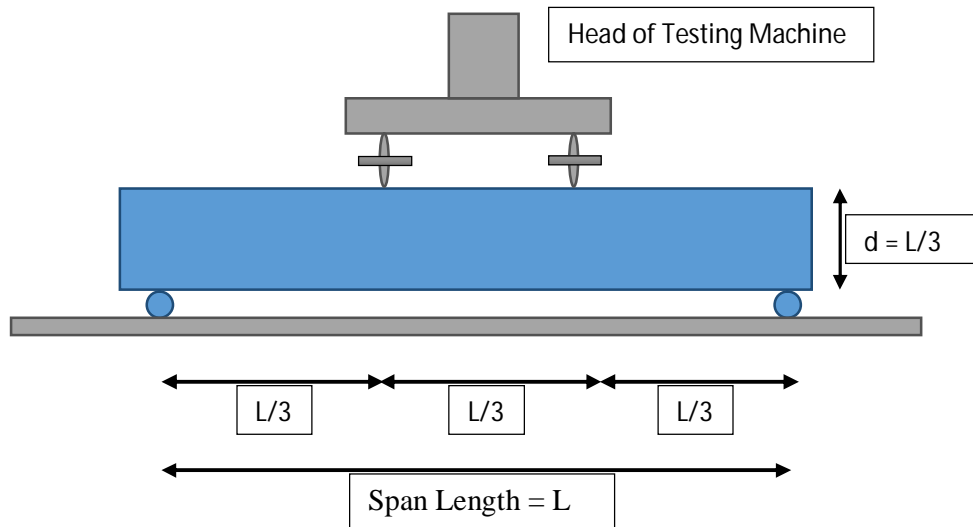
Figure 3.3 Four Point Loading
