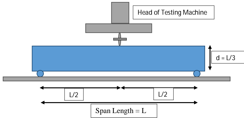
Figure 3.2 Centre Point Loading
